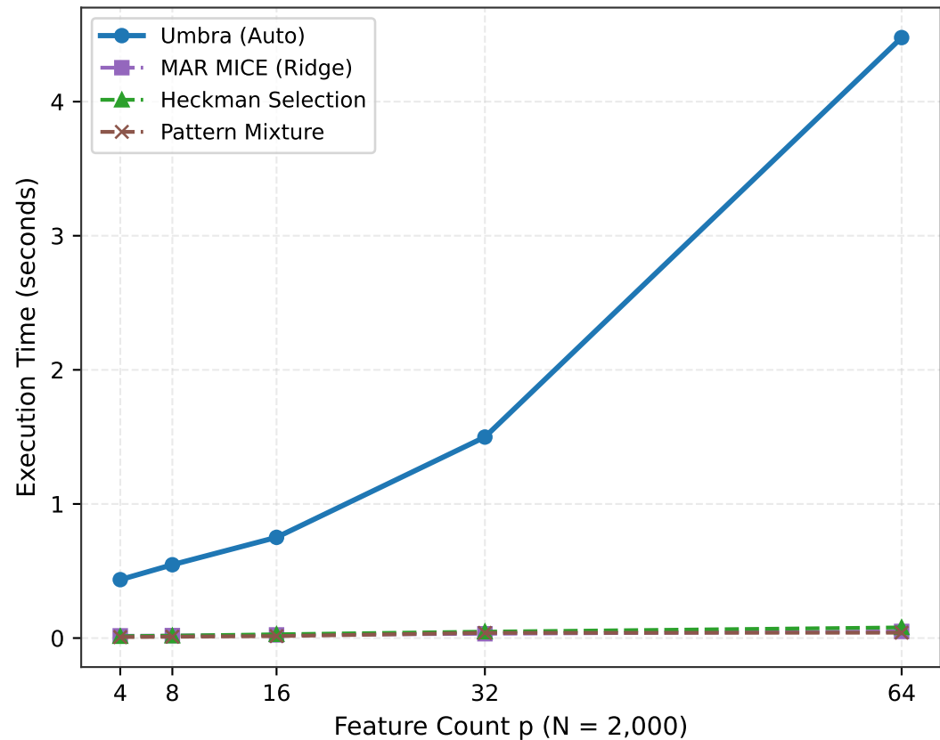
B: Runtime Scaling vs Feature Dimension p
