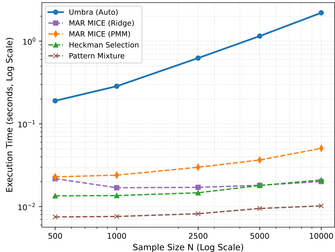
A: Runtime Scaling vs Sample Size N ( p = 5 )
