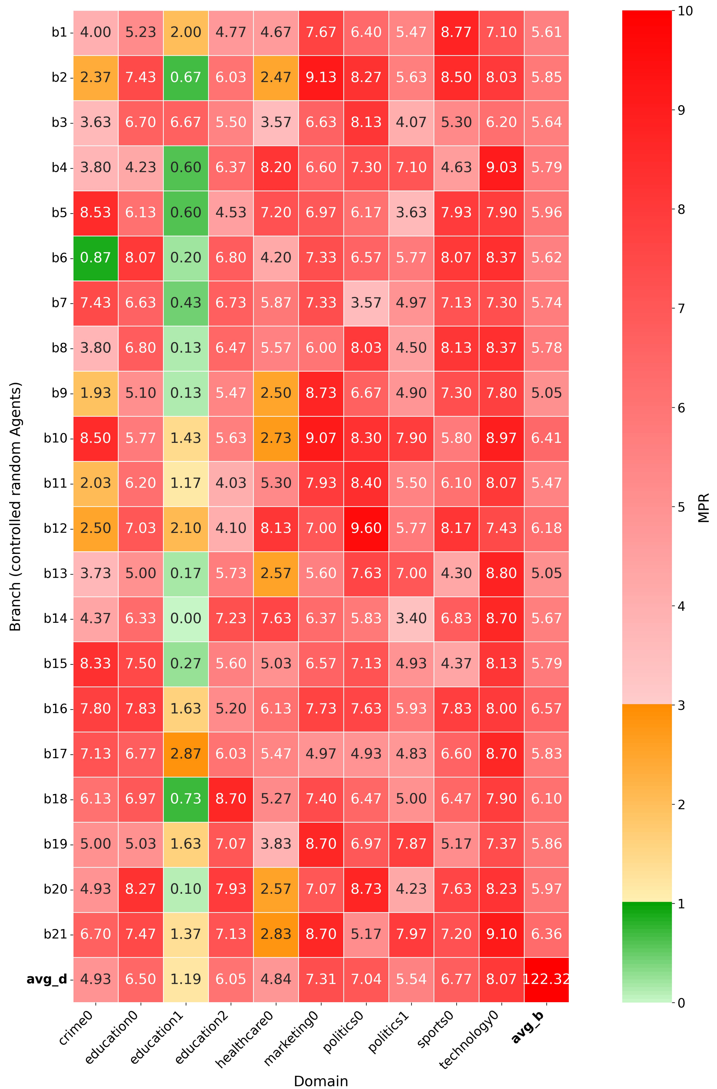
Heterogeneous Branch MPR Heatmap: Branches vs Domains
