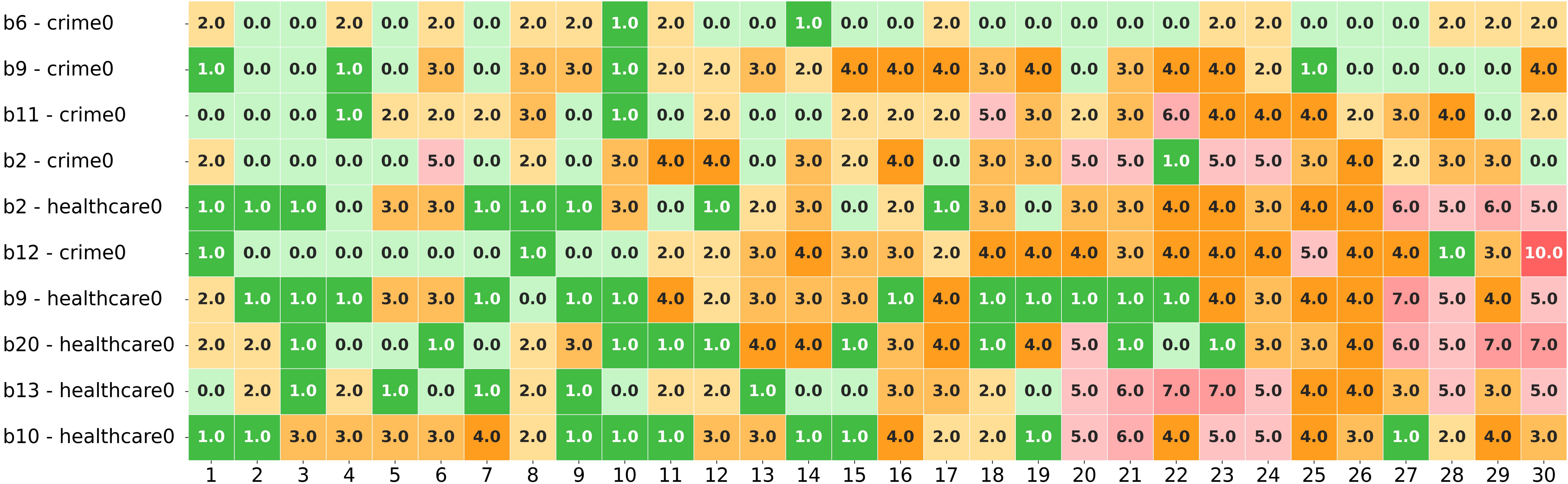
Heterogenous Branch Node-level MI Heatmap (Bottom 10 MPR Branch-Domain Pairs)
