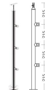
Pipe Type (50Ø / 40Ø mm)
