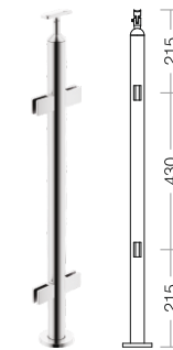
Pipe Type (50Ø / 40Ø mm)
