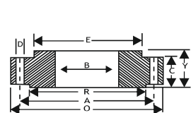
SLIP-ON FLANGE
