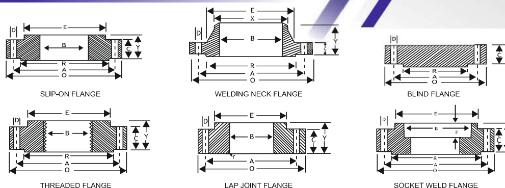
DIMENSIONS OF CLASS 1500 FLANGES AS PER B16.5
