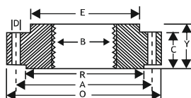
THREADED FLANGE
