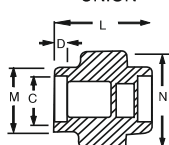
SOCKET WELD FITTING TO ANSI B-16.11
