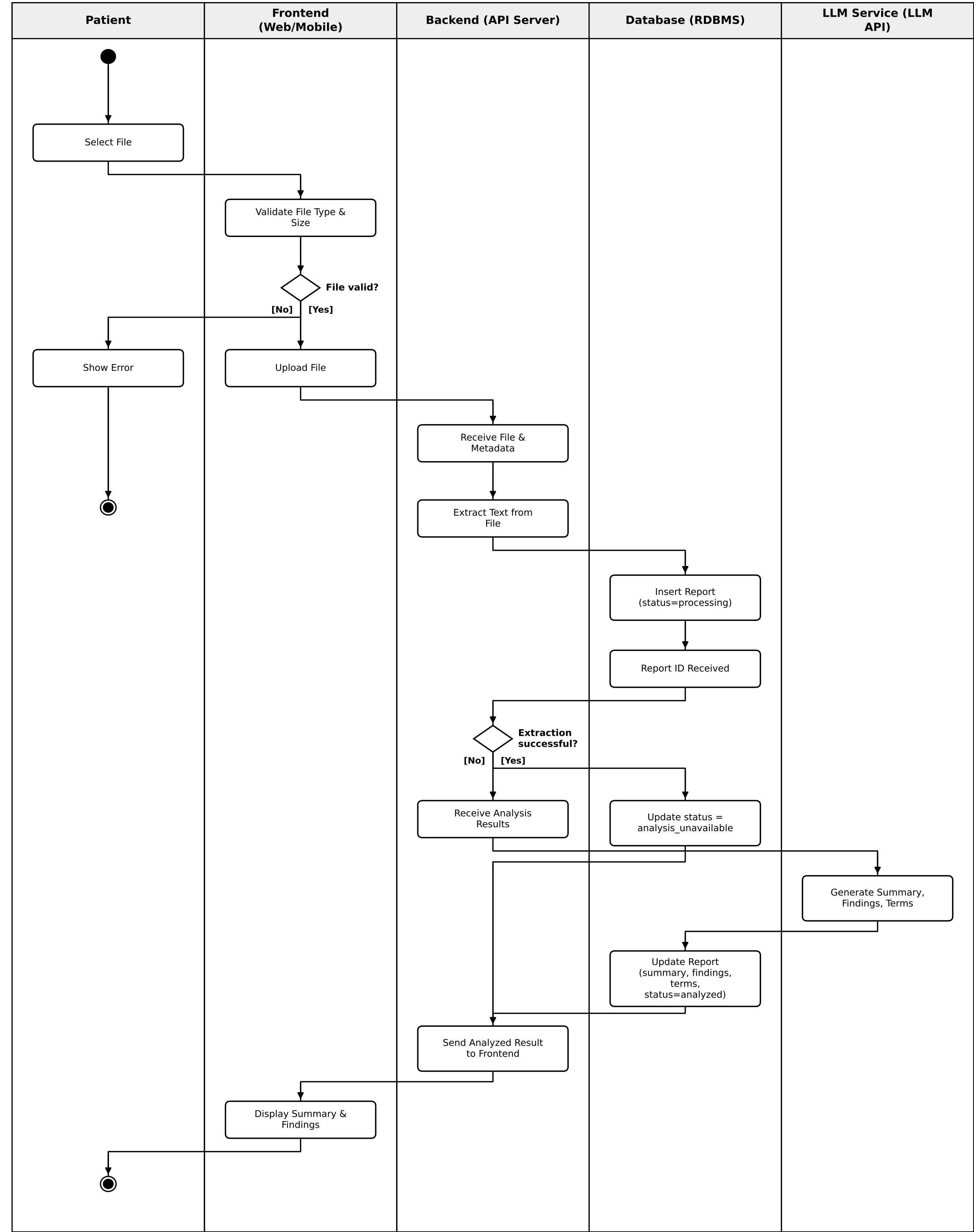
Activity Diagram 1 - Report Upload and AI Analysis
