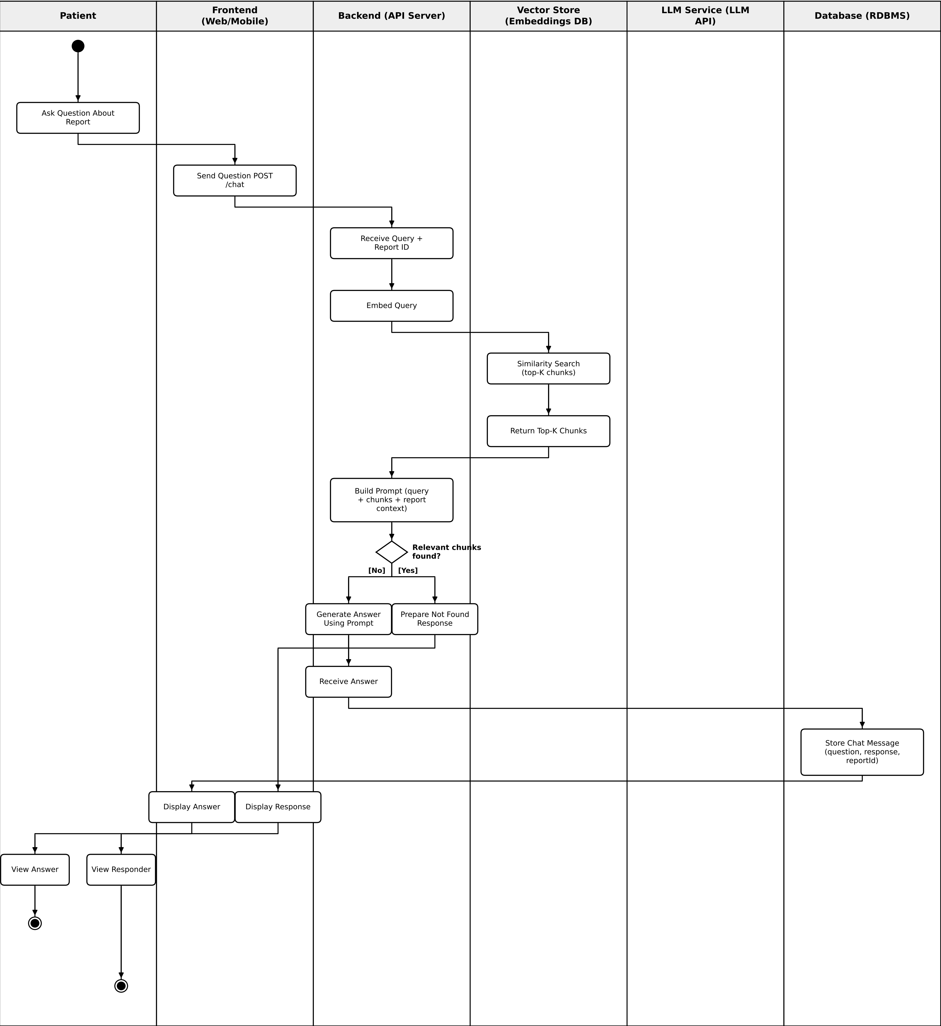
Activity Diagram 2 - AI Chat / RAG-based Q&A
