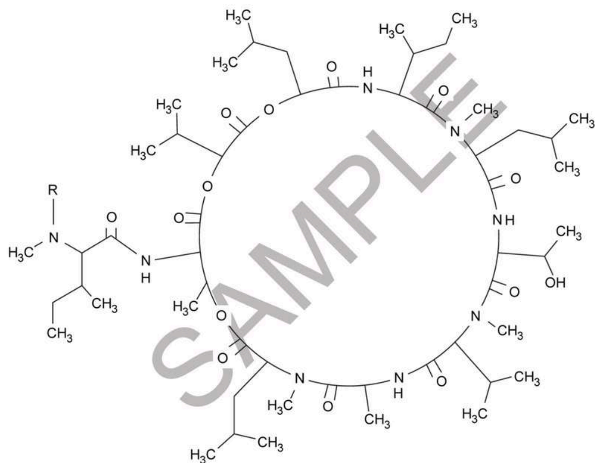
Chemical Structure
