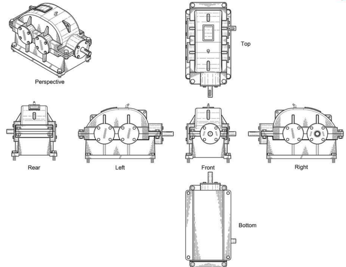
Mechanical Gearbox
