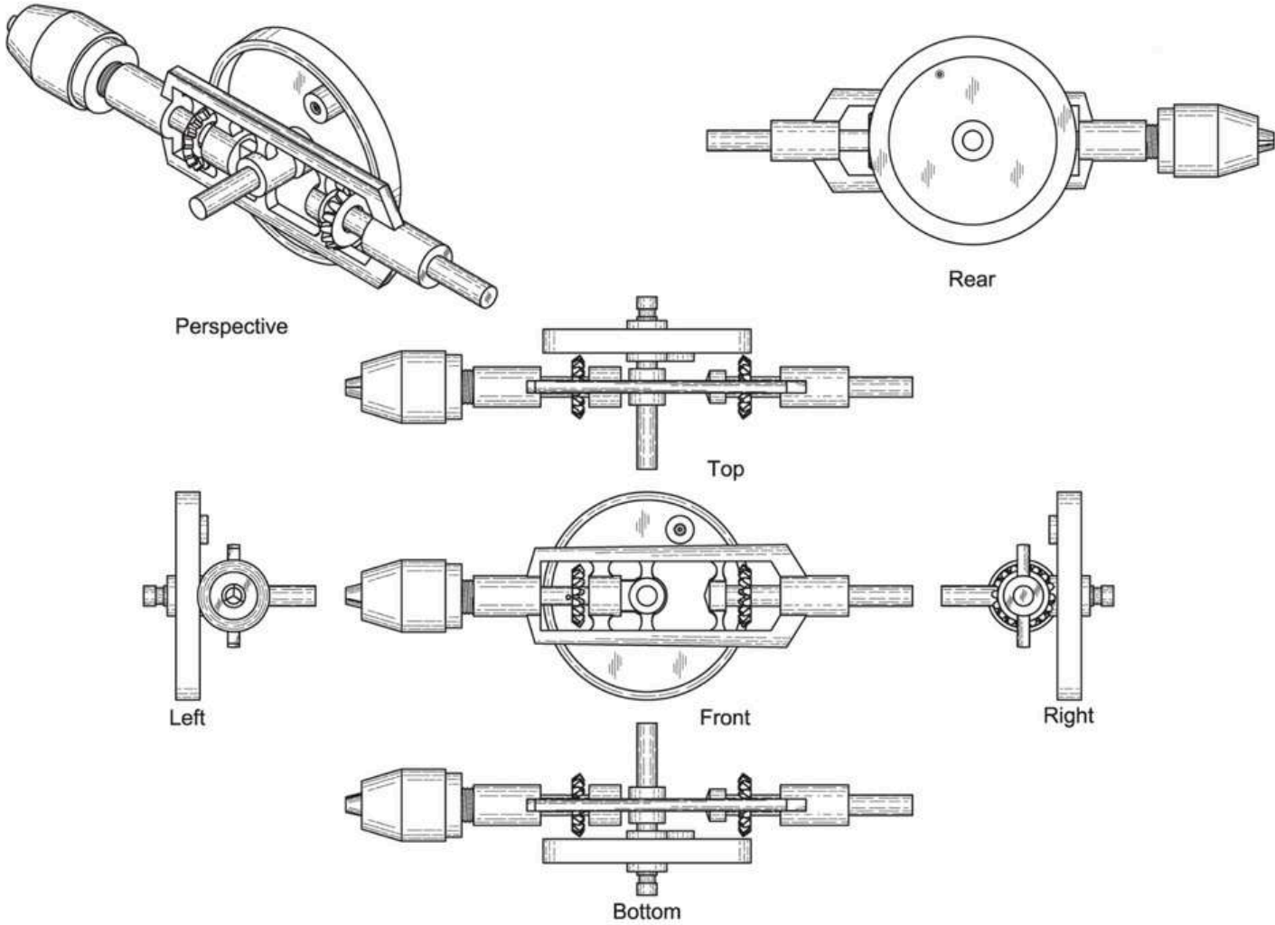
Manual Hand Drill
