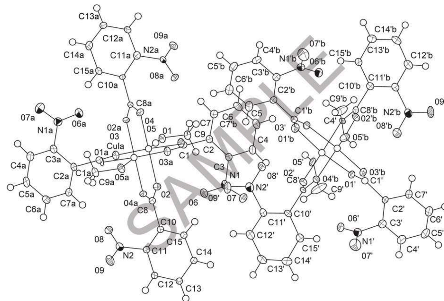
Chemical Structure
