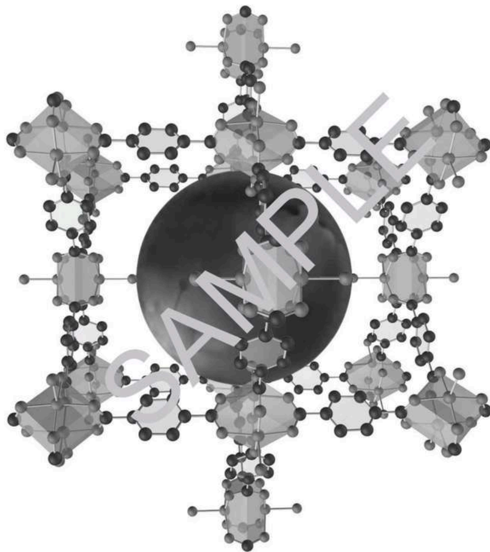
Chemical Structure
