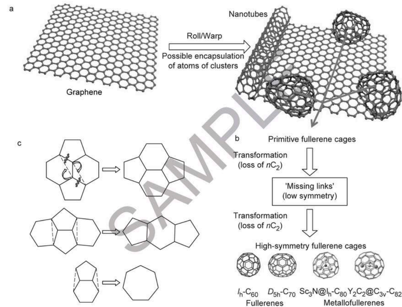
Chemical Structure
