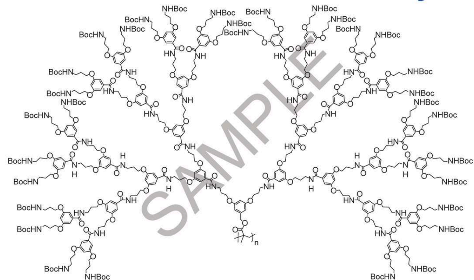
Chemical Structure
