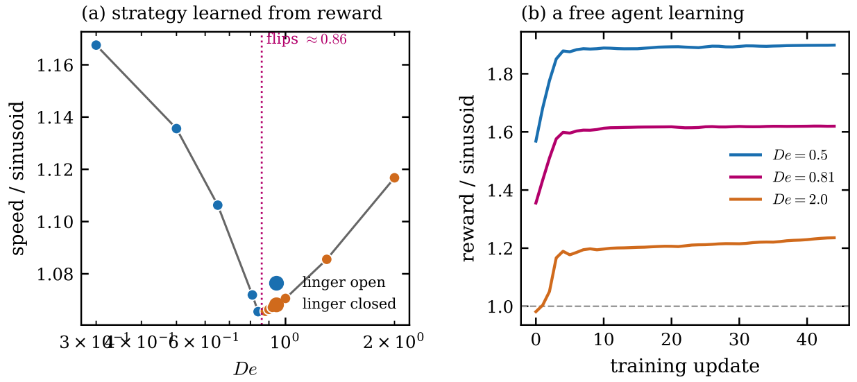
Figure 5. Reinforcement learning. (a) The strategy an agent learns from reward alone at each fluid; colour is the learned rhythm, which flips from open to closed at the crossover. (b) Learning curves: reward relative to the sinusoid, climbing as the agent learns.
