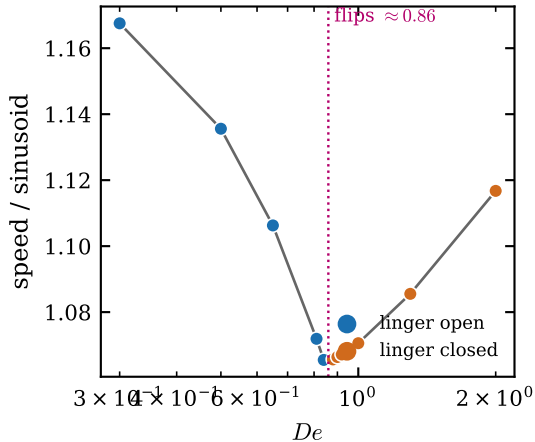
(a) strategy learned from reward
