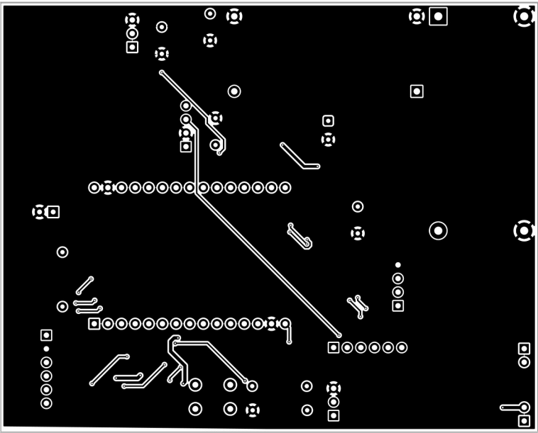
BACK (BOTTOM) LAYER Bottom Traces & B.Cu Plane
