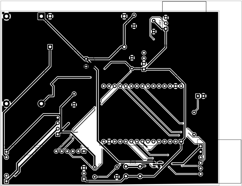
FRONT (TOP) LAYER Components, Silkscreen & F.Cu
