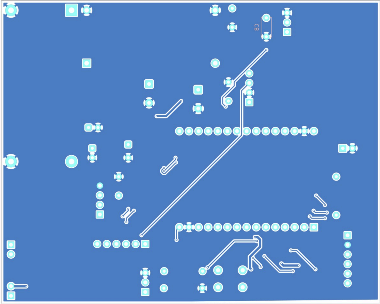
BACK (BOTTOM) LAYER Bottom Traces & B.Cu Plane
