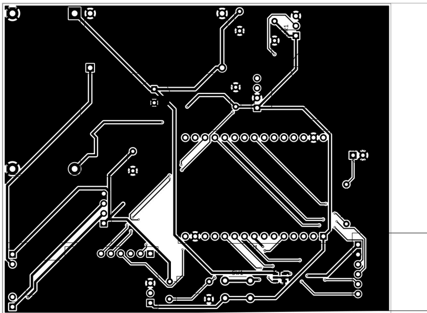
FRONT (TOP) LAYER Components, Silkscreen & F.Cu
