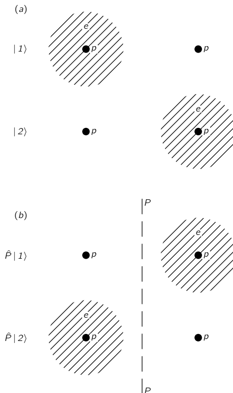
Fig. 17-1. If the states |1\rangle and |2\rangle are reflected in the plane P , they go into |2\rangle and |1\rangle , respectively.
