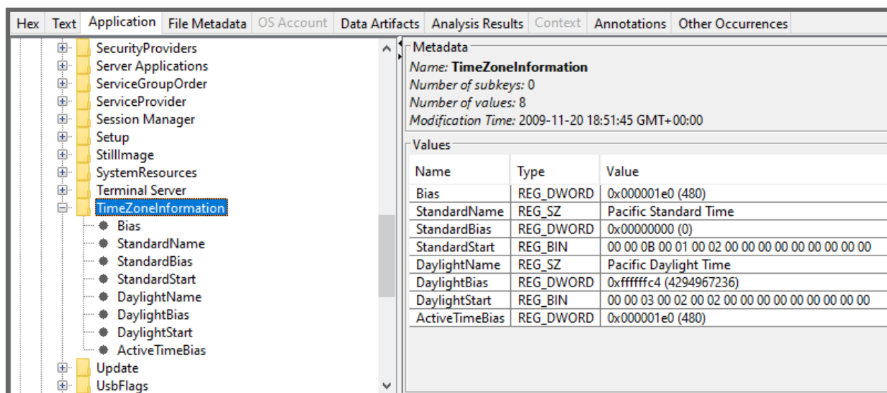
Registry Explorer: TimeZoneInformation key
