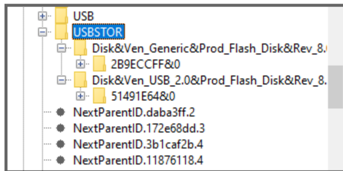
USBSTOR key with both devices
