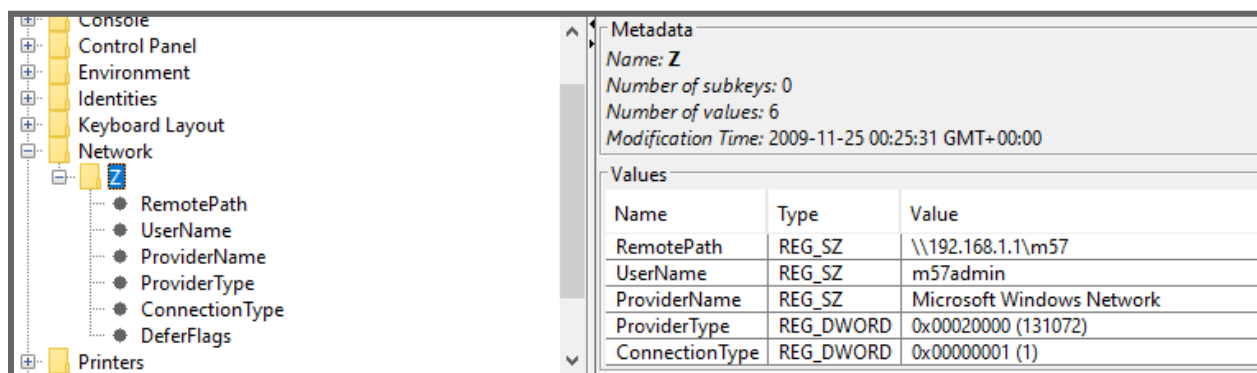
NTUSER.DAT \Network\Z key showing m57admin
