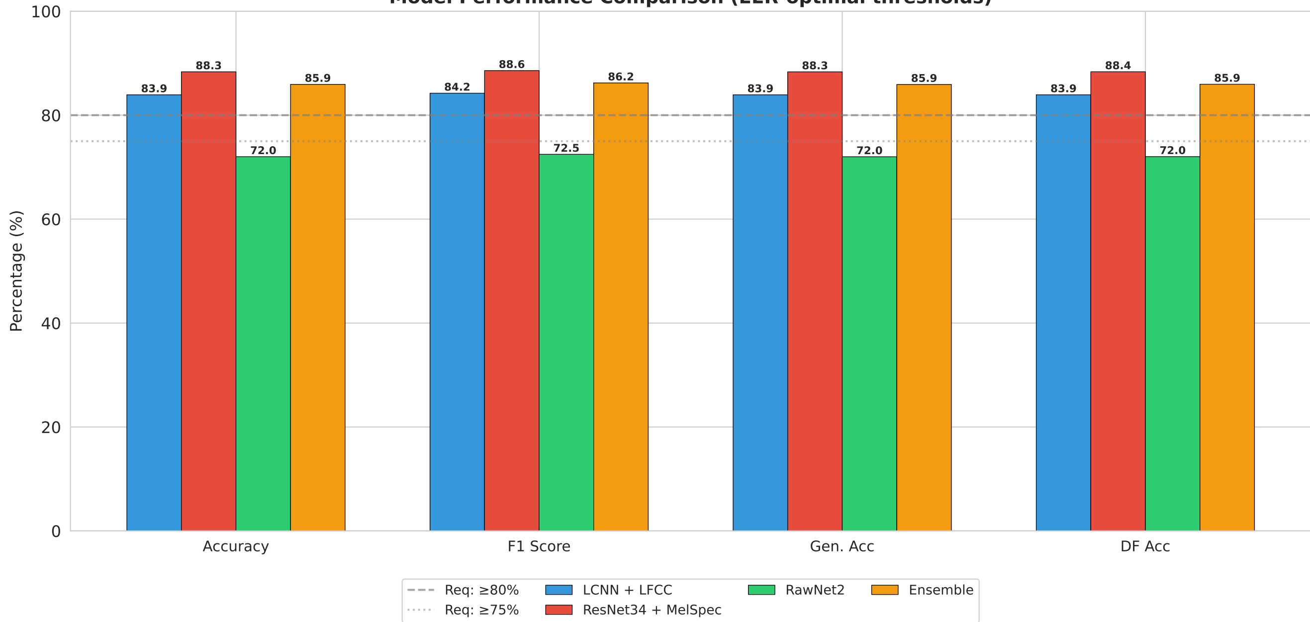
Model Performance Comparison (EER-optimal thresholds)
