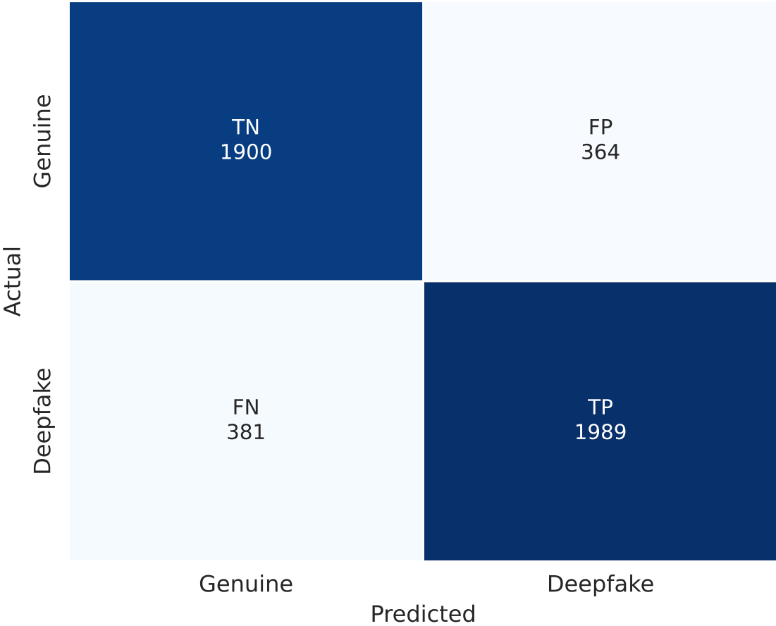
LCNN + LFCC Acc=83.9% | EER=16.1% | F1=84.2%
