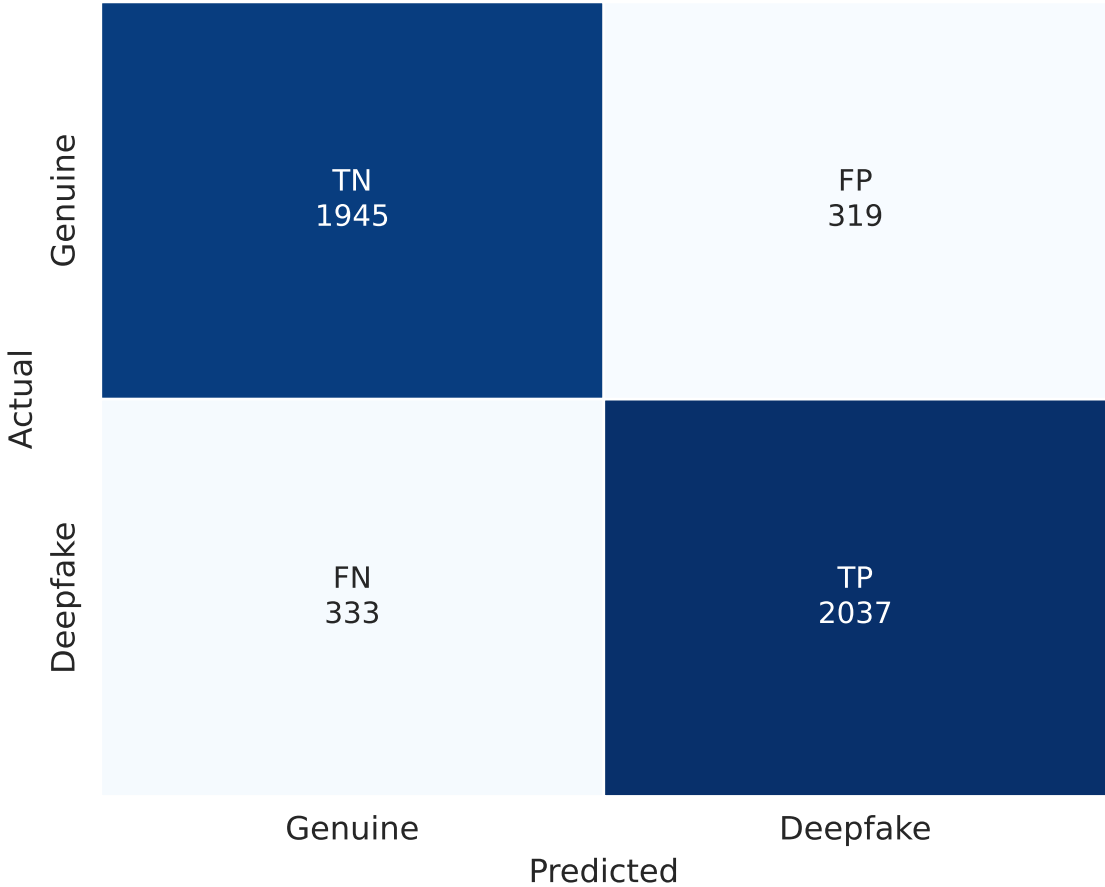
Ensemble Acc=85.9% | EER=14.1% | F1=86.2%
