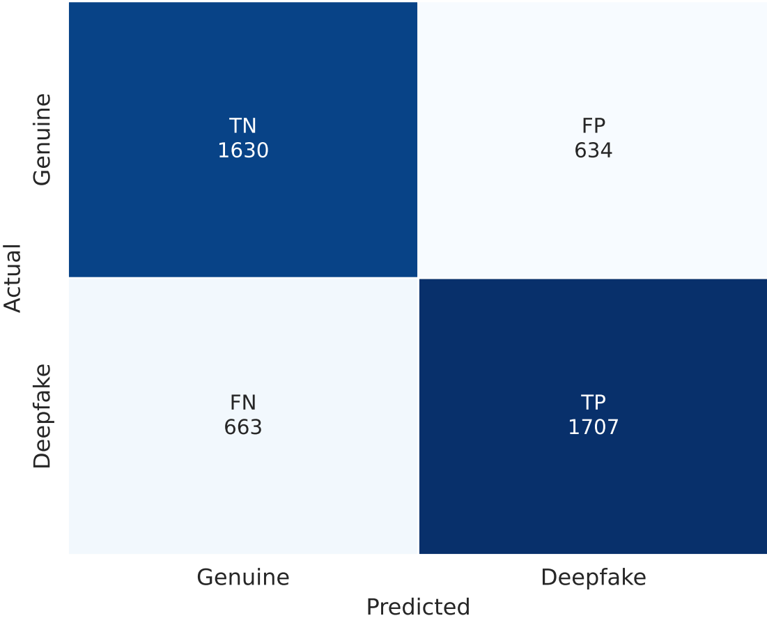
RawNet2 Acc=72.0% | EER=28.0% | F1=72.5%
