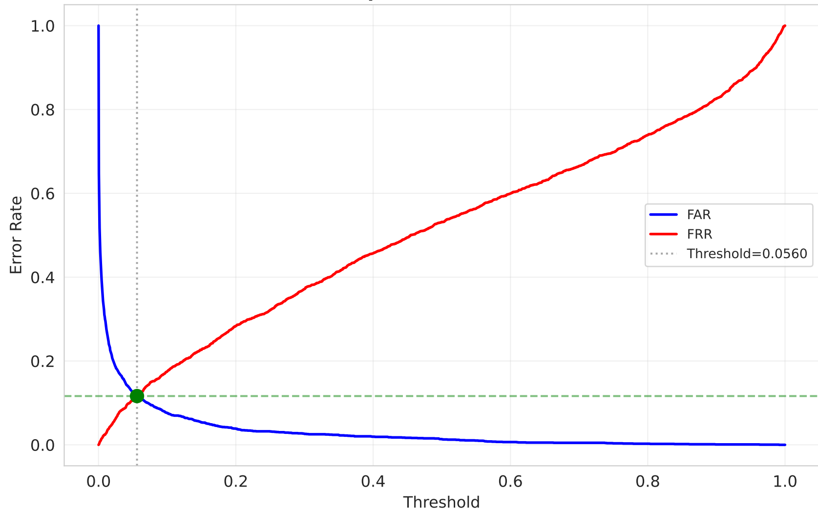
ResNet34 + MelSpec — EER Curve (EER = 11.6%)
