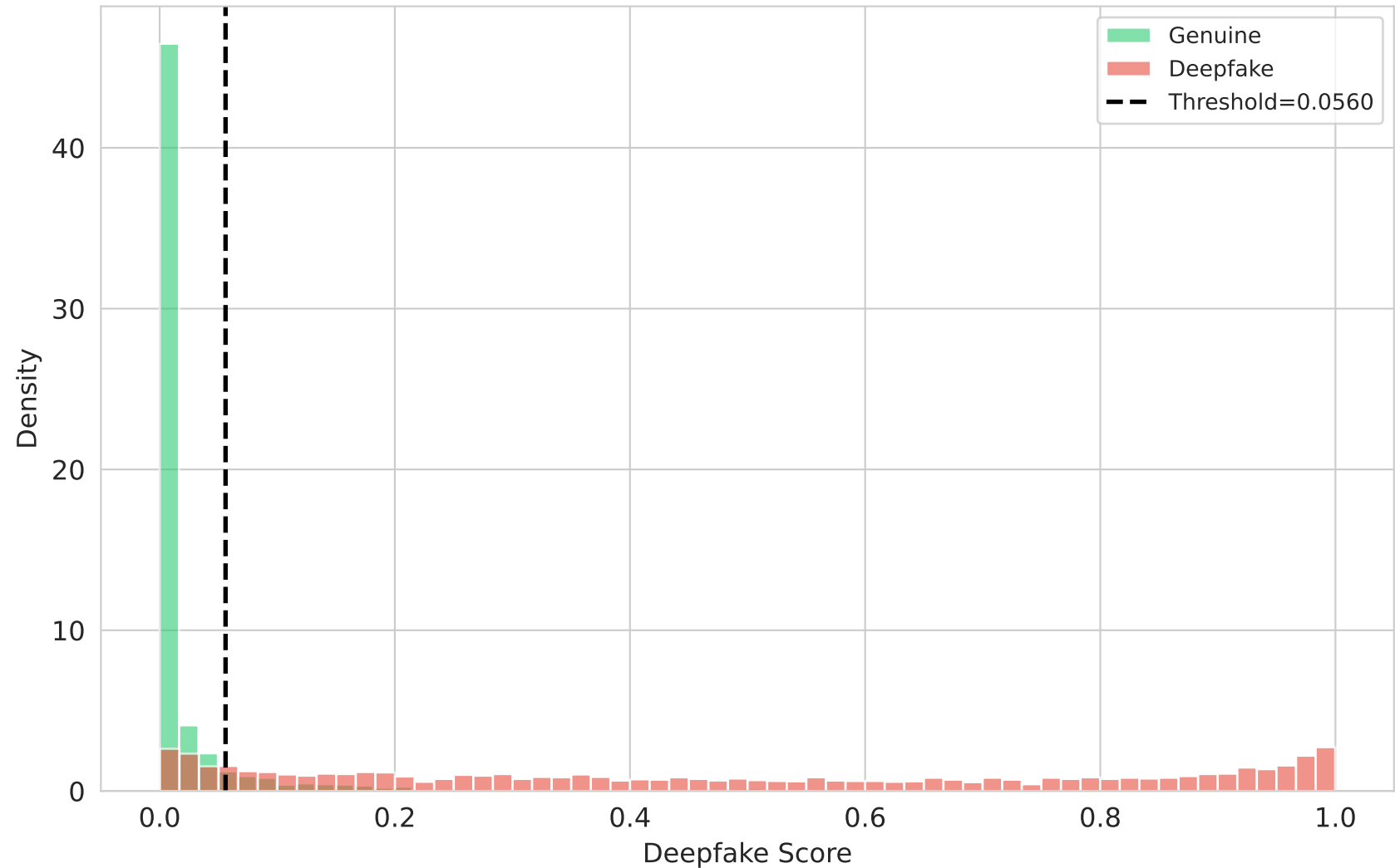
ResNet34 + MelSpec — Score Distribution
