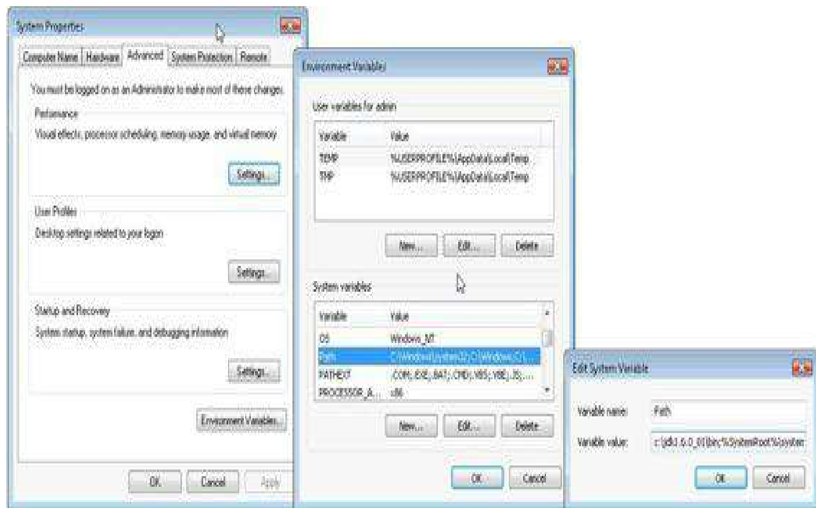
Figure 2.2. Setting the Path environment variable in Windows Vista
