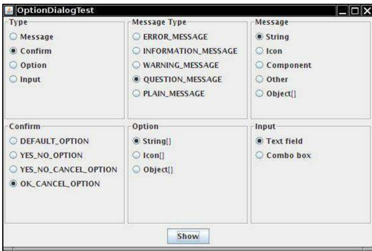
Figure 9.37. The OptionDialogTest program
