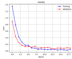
(b) Loss vs. Epochs
