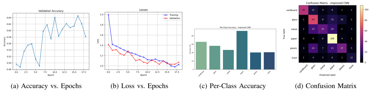
Fig. 2: Custom CNN results on TrashNet: (a) Accuracy vs. Epochs, (b) Loss vs. Epochs, (c) Per-Class Accuracy, (d) Confusion Matrix
