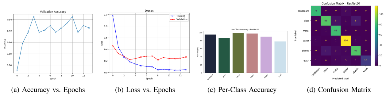
Fig. 3: ResNet-50 results on TrashNet: (a) Accuracy vs. Epochs, (b) Loss vs. Epochs, (c) Per-Class Accuracy, (d) Confusion Matrix
