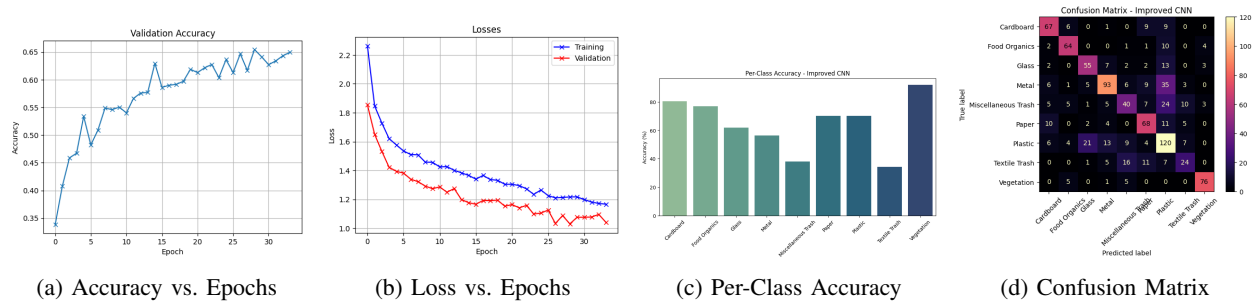
Fig. 4: Custom CNN results on RealWaste: (a) Accuracy vs. Epochs, (b) Loss vs. Epochs, (c) Per-Class Accuracy, (d) Confusion Matrix
