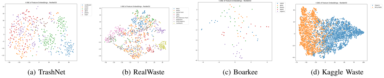
Fig. 10: ResNet-50 t-SNE Feature Visualizations across datasets: (a) TrashNet, (b) RealWaste, (c) Boarkee, (d) Kaggle Waste.
