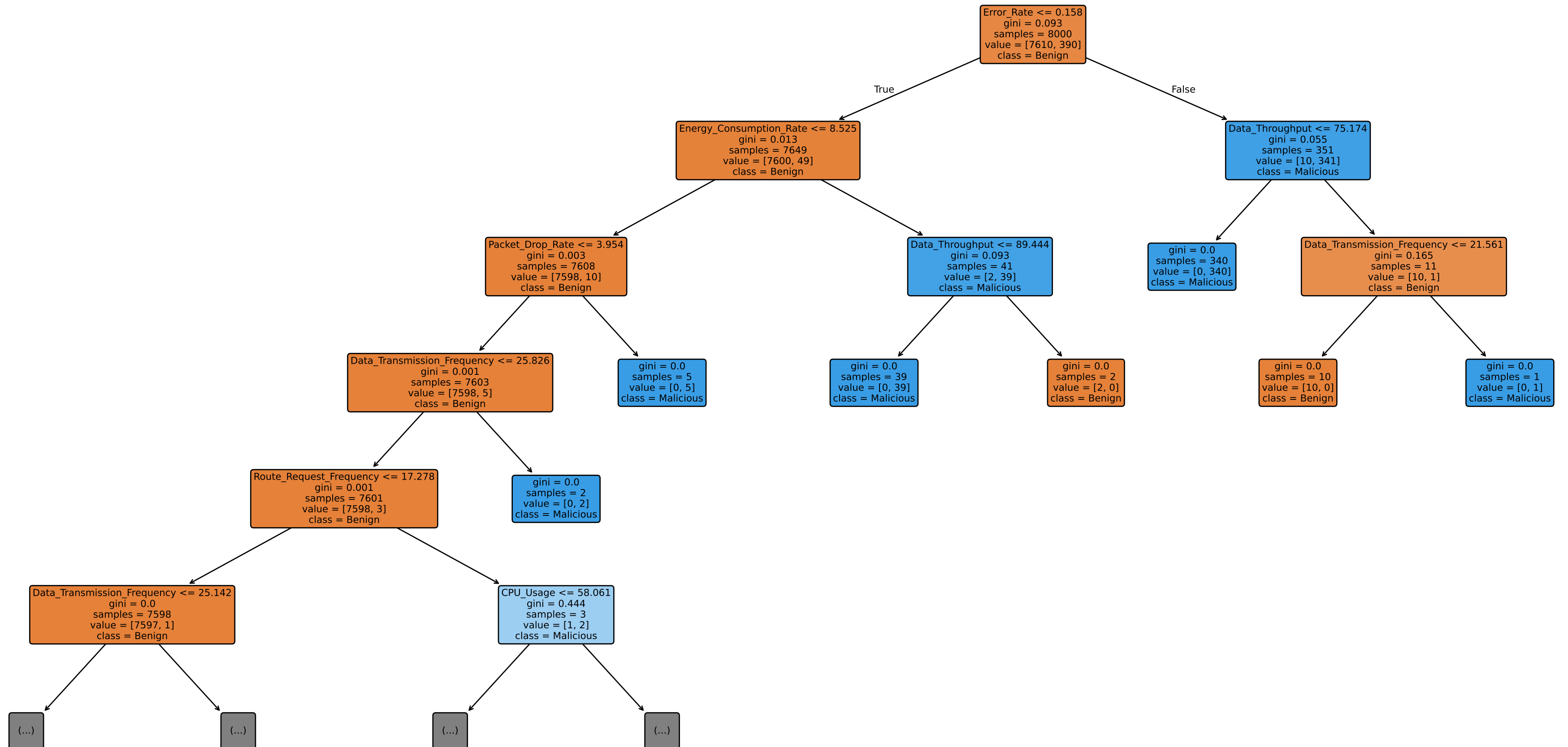
Decision Tree Visualization (max_depth=5) - SensorNetGuard
