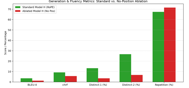
(b) Standard Attention (RoPE) vs. Ablated Attention (No Positional Embeddings)
