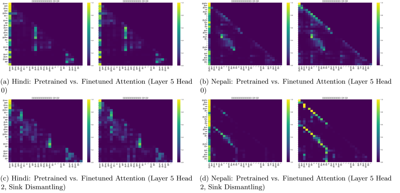
Figure 5: High-resolution Pretrained vs. Supervised Finetuned attention maps on reasoning prompts across Hindi and Nepali. Finetuning visibly sharpens relational focus (contracting receptive token distance in L5H0) and dismantles pathological token-0 sinks (redirecting attention mass to entity tokens in L5H2).
