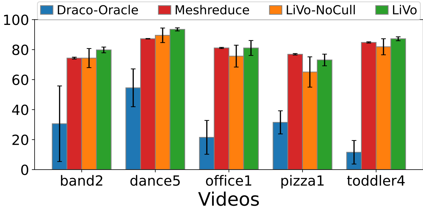
PSSIM Color
