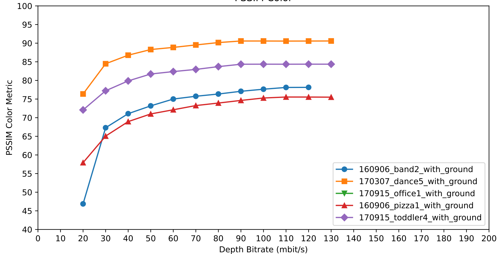
PSSIM Color
