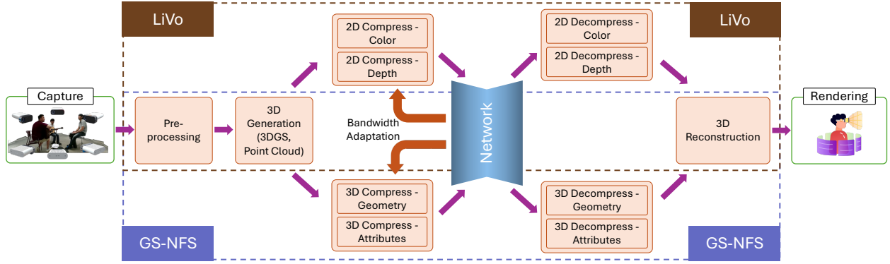
FIGURE 1.3: The dissertation’s vision for volumetric communication. LiVo and GS-NFS address complementary paths through a common end-to-end delivery pipeline.
