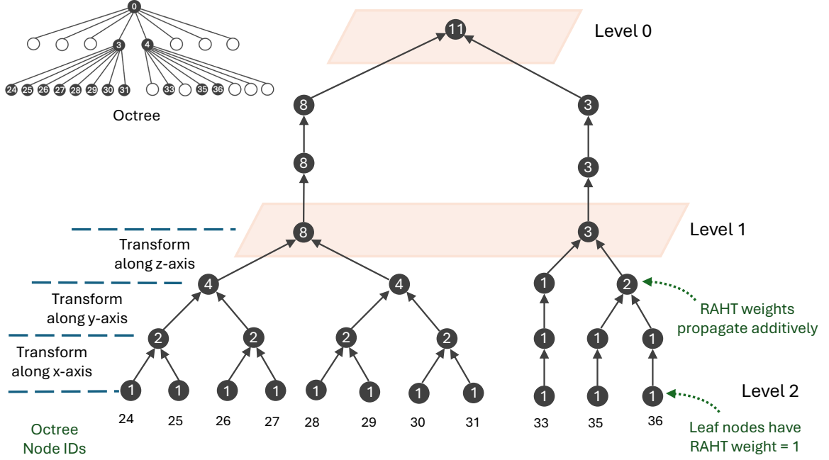
FIGURE 3.4: Example to illustrate the RAHT algorithm.
