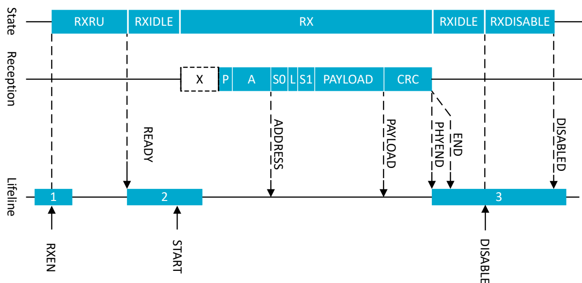
Figure 100: Receive sequence
