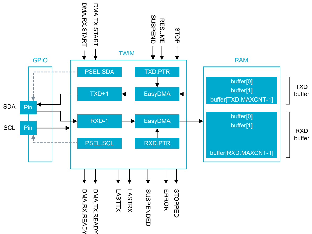
Figure 154: TWIM with EasyDMA
