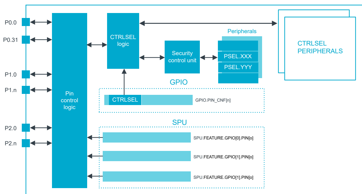
Figure 30: Pin access using CTRLSEL
