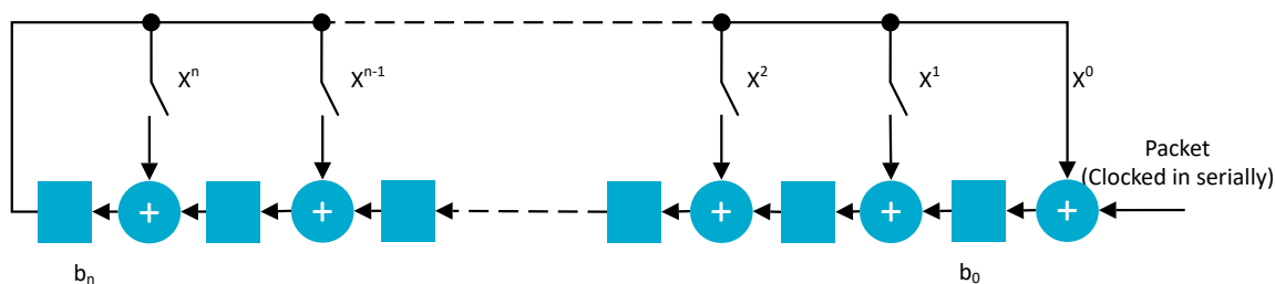
Figure 94: n bit CRC generation
