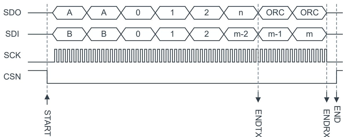
Figure 118: SPIM transaction
