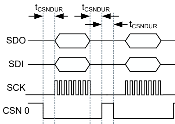
Figure 120: CSNDUR example
