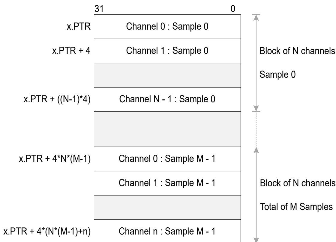
Figure 152: Memory mapping for 32 bit TDM. CONFIG.SWIDTH = 32Bit, CONFIG.CHANNEL.NUM = n and all channels enabled in CONFIG.CHANNEL.MASK
