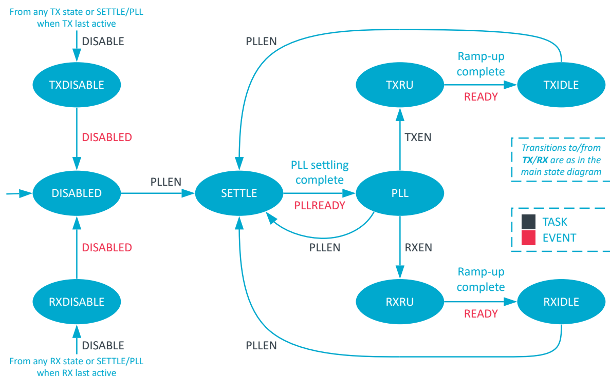
Figure 96: Radio states, PLL only
