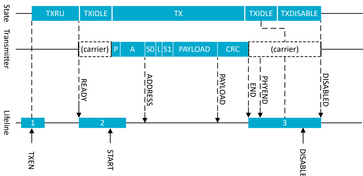
Figure 97: Transmit sequence
