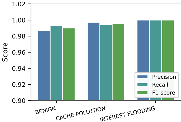
NDN PoC — Per-Class Metrics (held-out)
