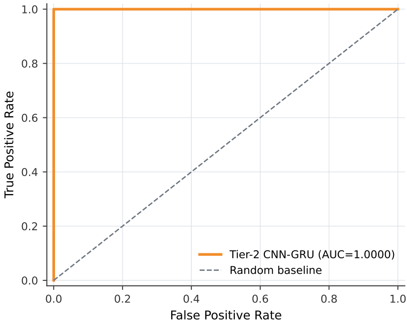
Tier-2 Attack Detection ROC
