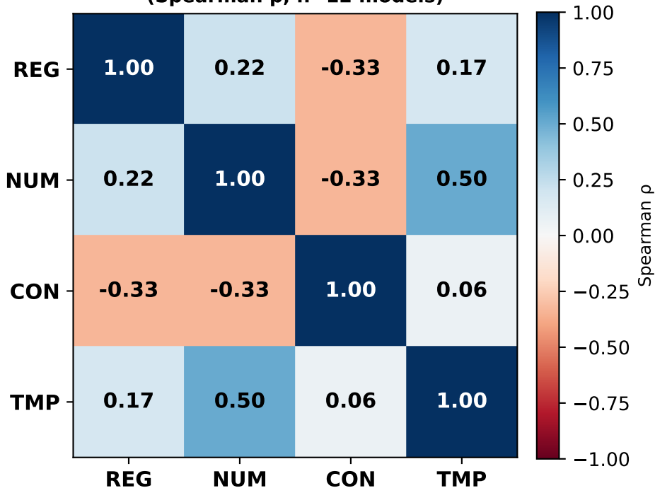
Inter-Task Correlation (Spearman \rho , n=12 models)
