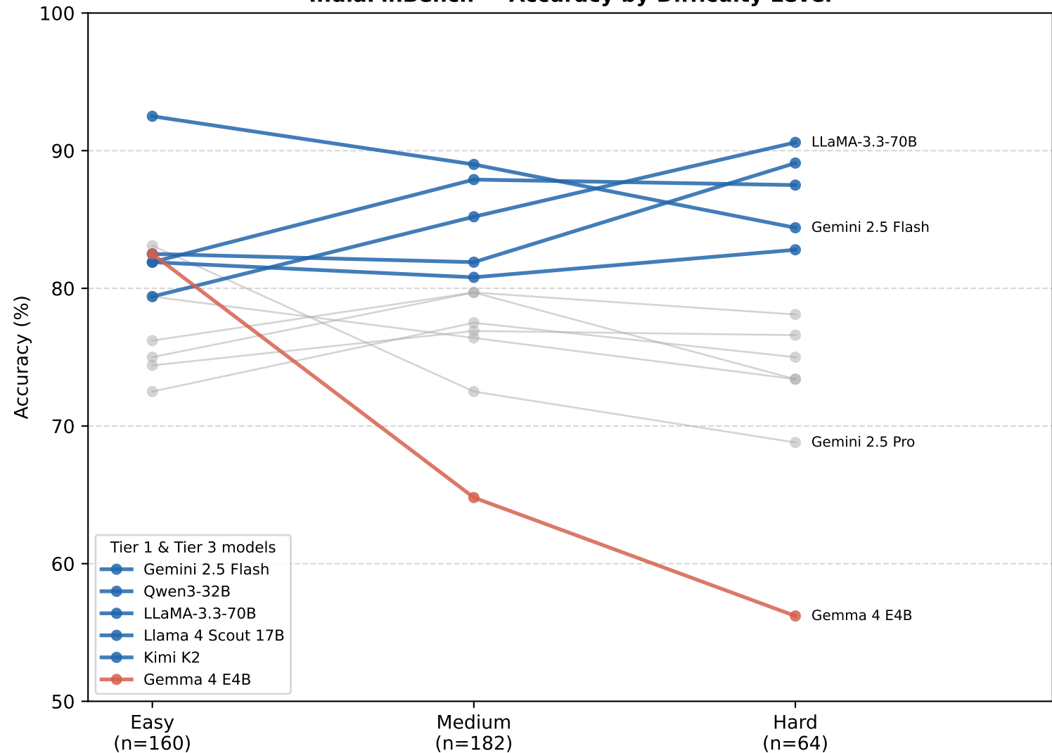
IndiaFinBench — Accuracy by Difficulty Level
