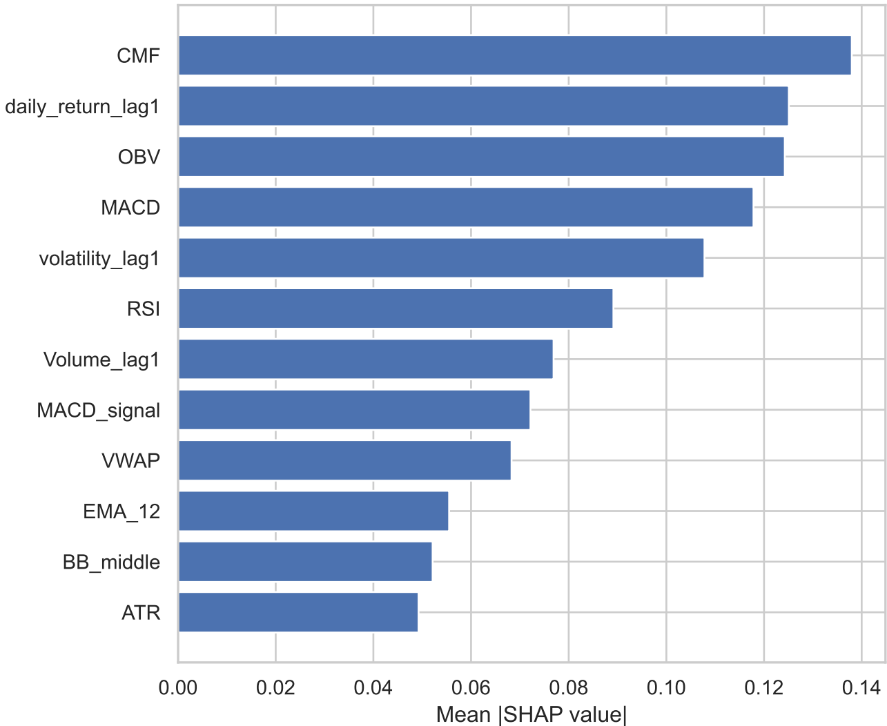
Figure 3 — SHAP Feature Importance
