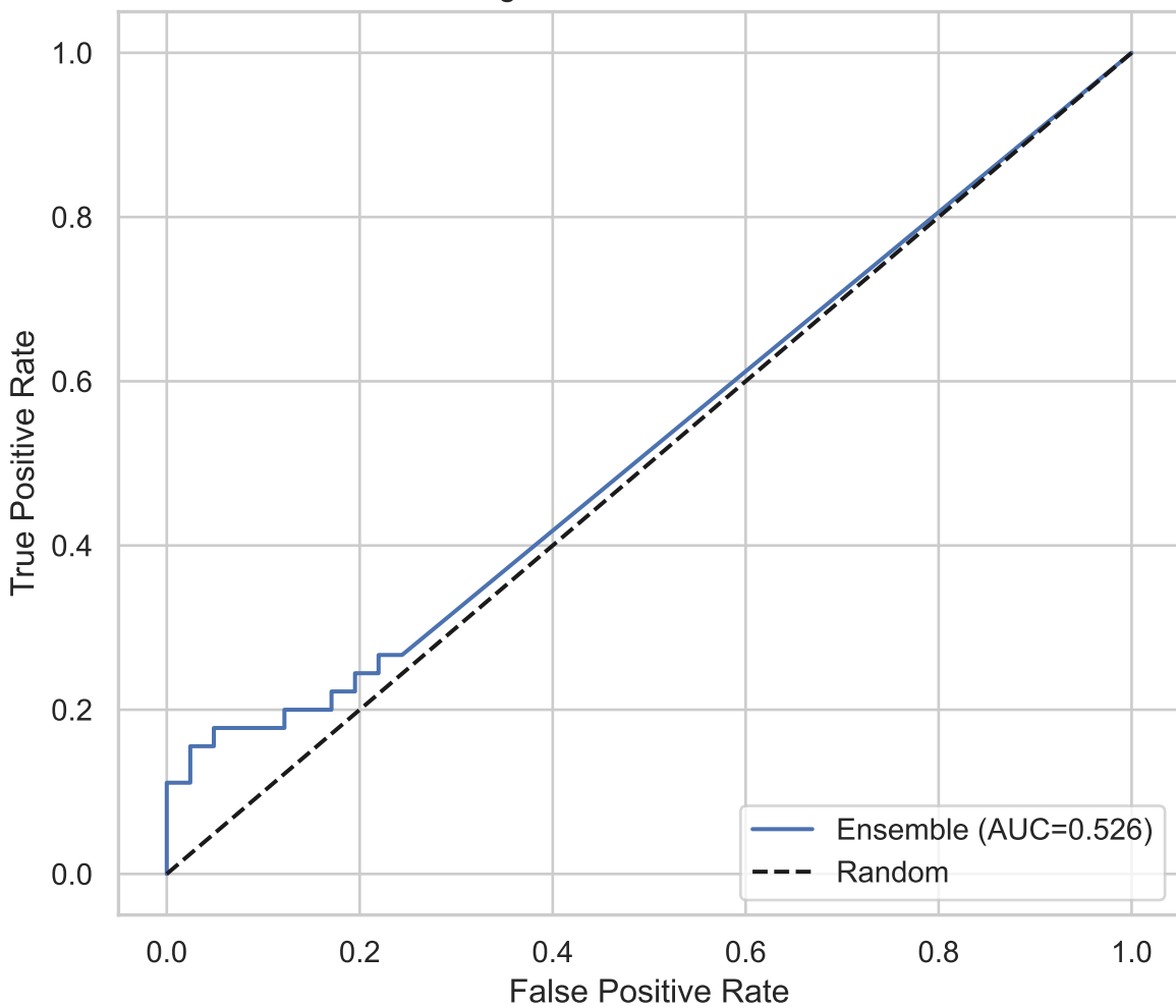
Figure 5 — ROC Curves
