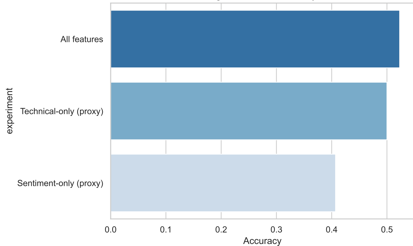
Figure 7 — Ablation Study
