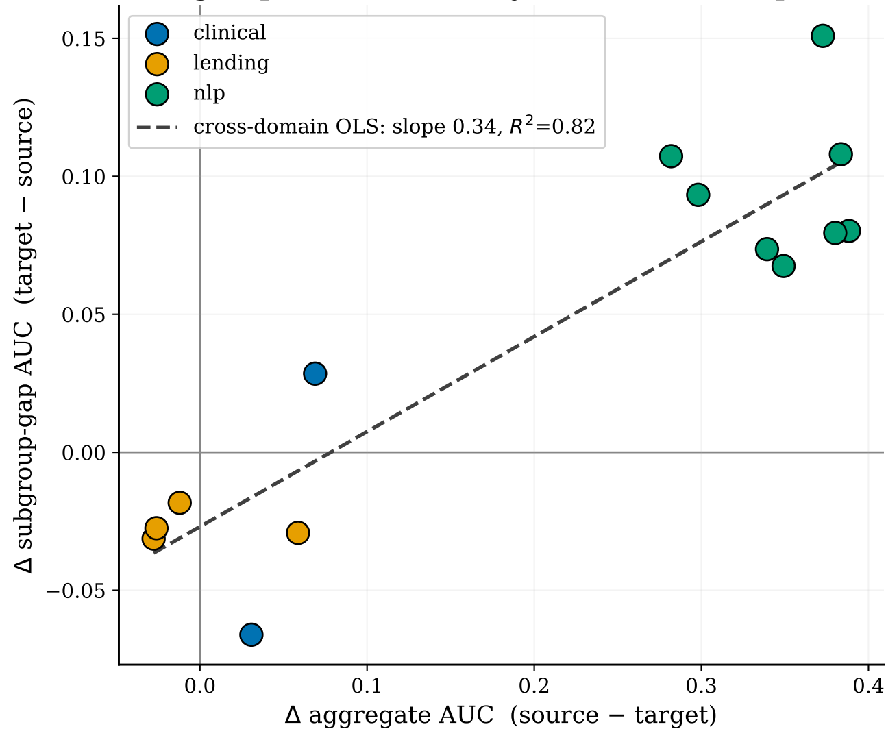
Subgroup loss vs. accuracy loss across shift-points
