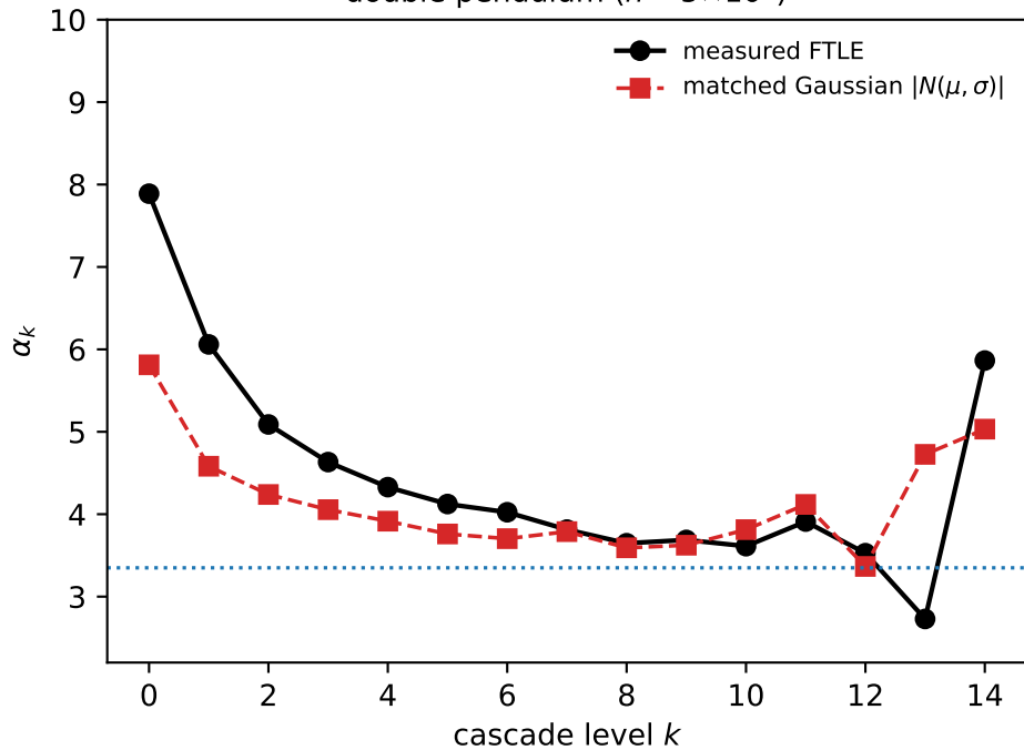
double pendulum ( n = 5 \times 10^5 )
