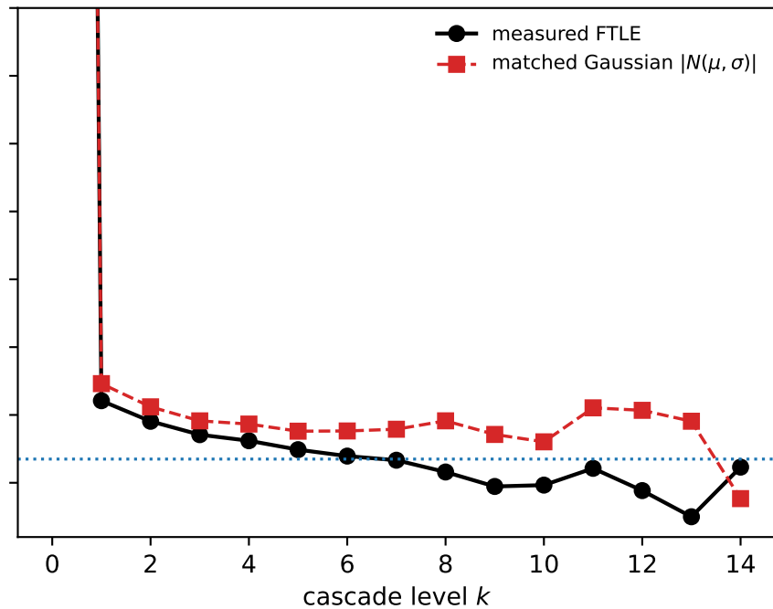
Lorenz-63 ( n = 5 \times 10^5 )
