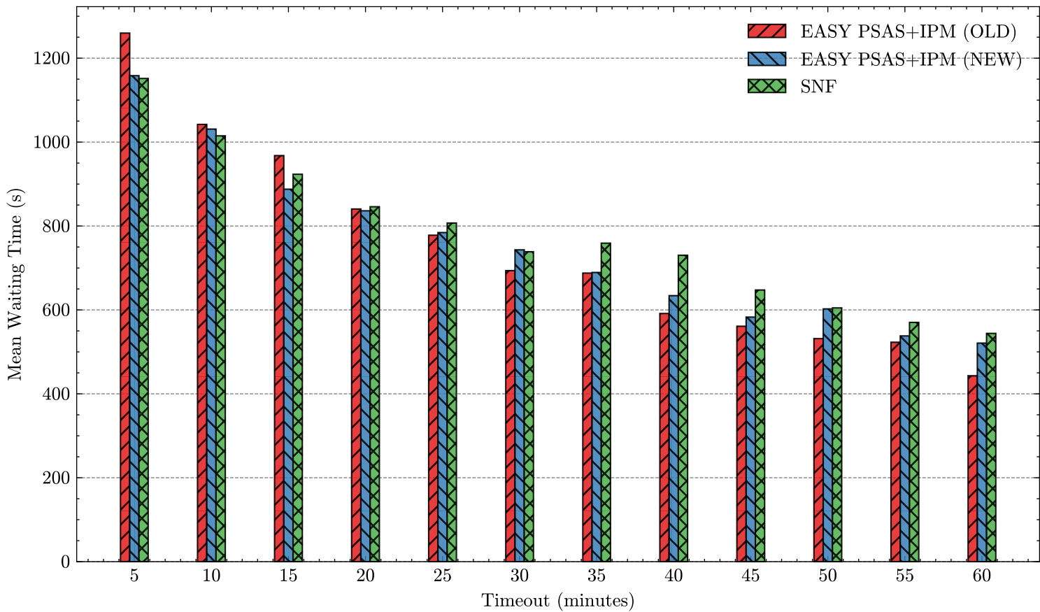
Mean Waiting Time vs Timeout
