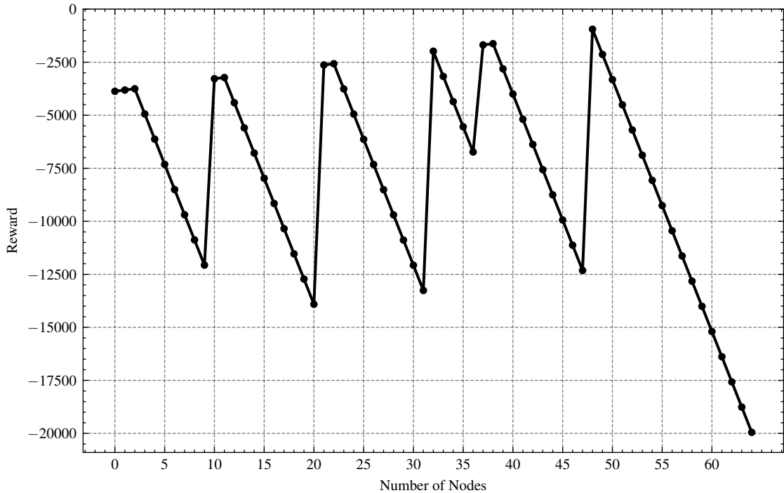
Reward vs Number of Nodes
