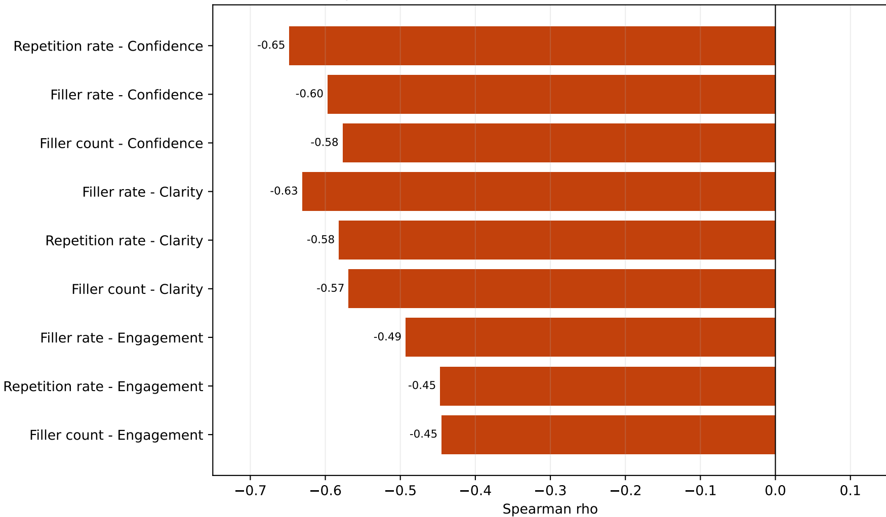
Top Feature Correlations with Human Reference Scores
