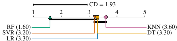
(a) COCOMO81: Friedman p = 0.038
