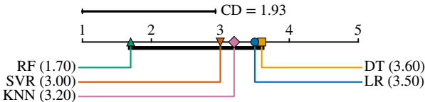
(b) NASA93: Friedman p = 0.053
