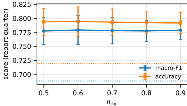
(a) stability threshold, B = 15
