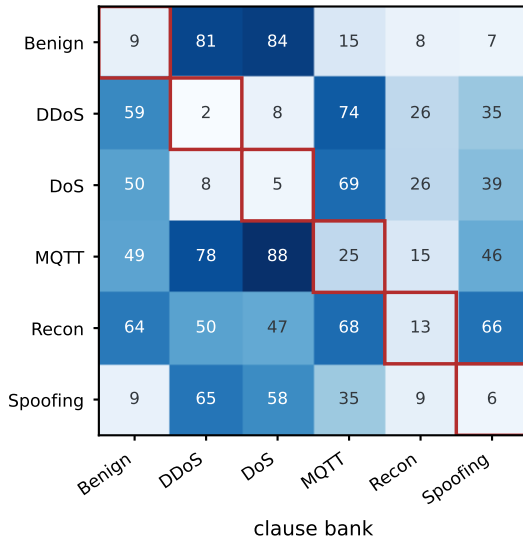
negative-polarity clauses (vote AGAINST their own class)
