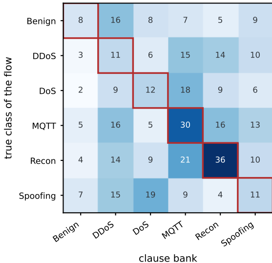
positive-polarity clauses (vote FOR their own class)
