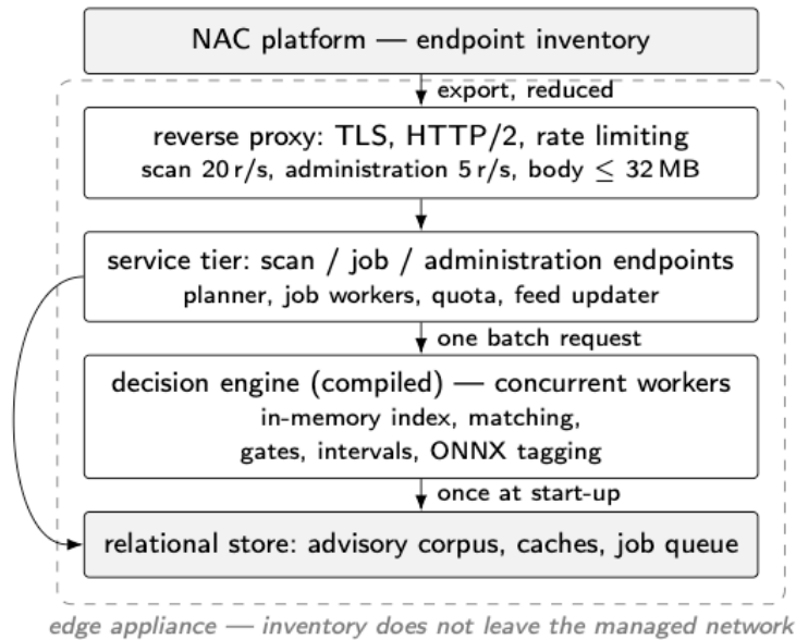
Figure 2. Deployment. The inventory is reduced where it is held, submitted once, and adjudicated inside the managed network.
