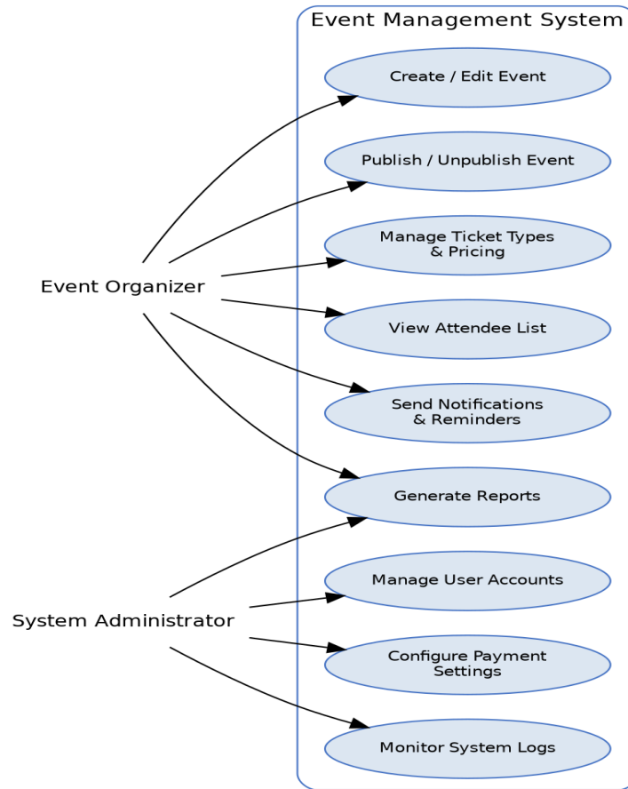
Figure 2: Use-case diagram for Event Organizer and System Administrator interactions.
