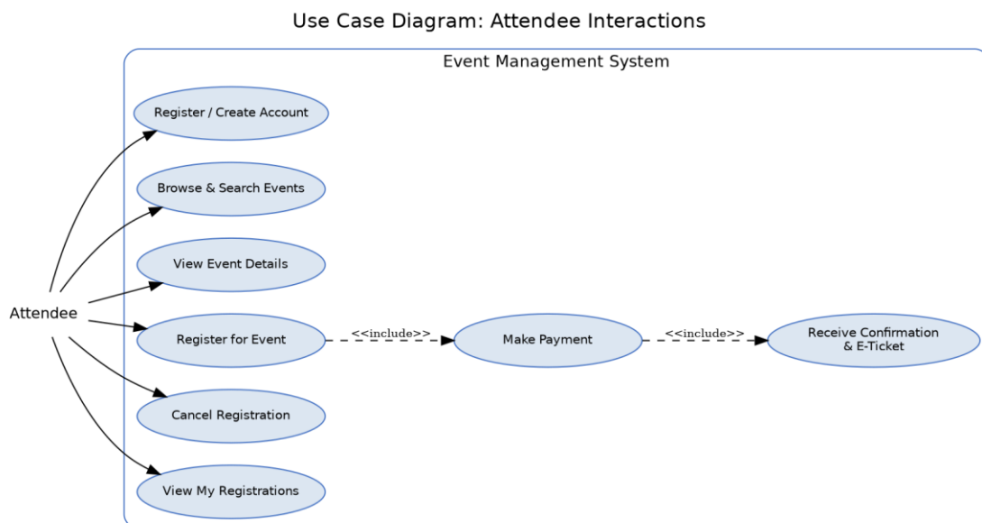
Figure 1: Use-case diagram for Attendee interactions.
