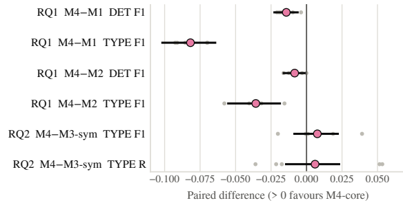
Figure 2: The six pre-declared tests. Pink: mean difference (M4-core minus baseline). Black bar: 95% CI. Grey: the five per-seed differences. All RQ1 bars lie left of zero (M4-core worse); both RQ2 bars cross zero (no detectable difference).
