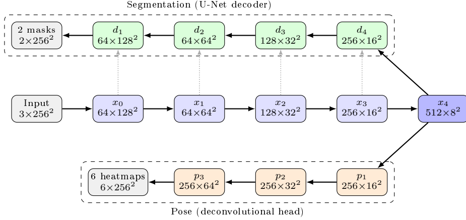
Fig. 1. HybridMTLNet architecture (channels \times spatial dimensions are indicated per block). A shared ResNet-34 encoder extracts multi-scale features x_0 – x_4 . The bottleneck representation x_4 feeds two parallel branches: a U-Net-based segmentation decoder ( d_4 – d_1 , with dotted lines denoting skip connections from the encoder) yielding two dense instance masks, and a deconvolutional pose head ( p_1 – p_3 ) yielding six key-point heatmaps (3 keypoints \times 2 instances). Both outputs are restored to the original 256 \times 256 resolution.
