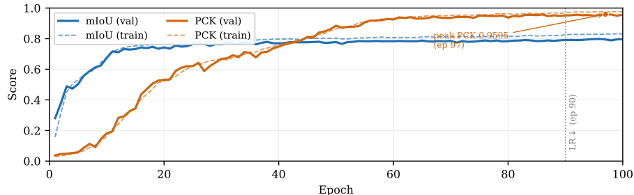
Fig. 4. Training dynamics of HybridMTLNet over 100 epochs (single 1:500 run). Segmentation mIoU converges quickly and saturates while pose PCK rises gradually; the dotted line marks the learning-rate decay at epoch 90, and the marker indicates the peak validation PCK (0.9595 at epoch 97).
