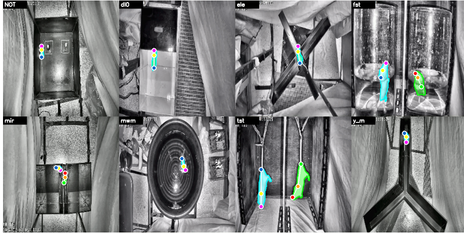
Fig. 2. Qualitative results across the eight behavioral paradigms. Each tile shows HybridMTLNet’s per-instance segmentation masks and keypoint skeletons (nose–shoulder–tail) on a held-out test image.
