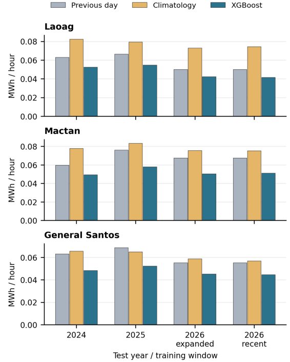
Fig. 7. Grid-plan adjustment per evaluated hour under the common 2 MWh battery replay. Normalization distinguishes full-year tests from partial 2026; units are MWh per hour.
