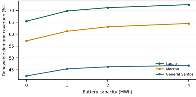
Fig. 3. Renewable coverage of the common synthetic demand by battery capacity. Stored energy is carried between hours.
