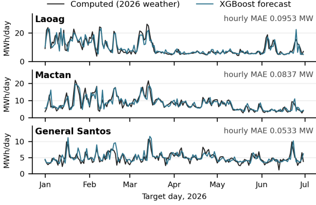
Fig. 6. January-June 2026 daily energy computed from 2026 weather versus XGBoost forecasts issued at 00:00 by models trained only on 2020-2025 data (last target 31 December 2025, 23:00).
