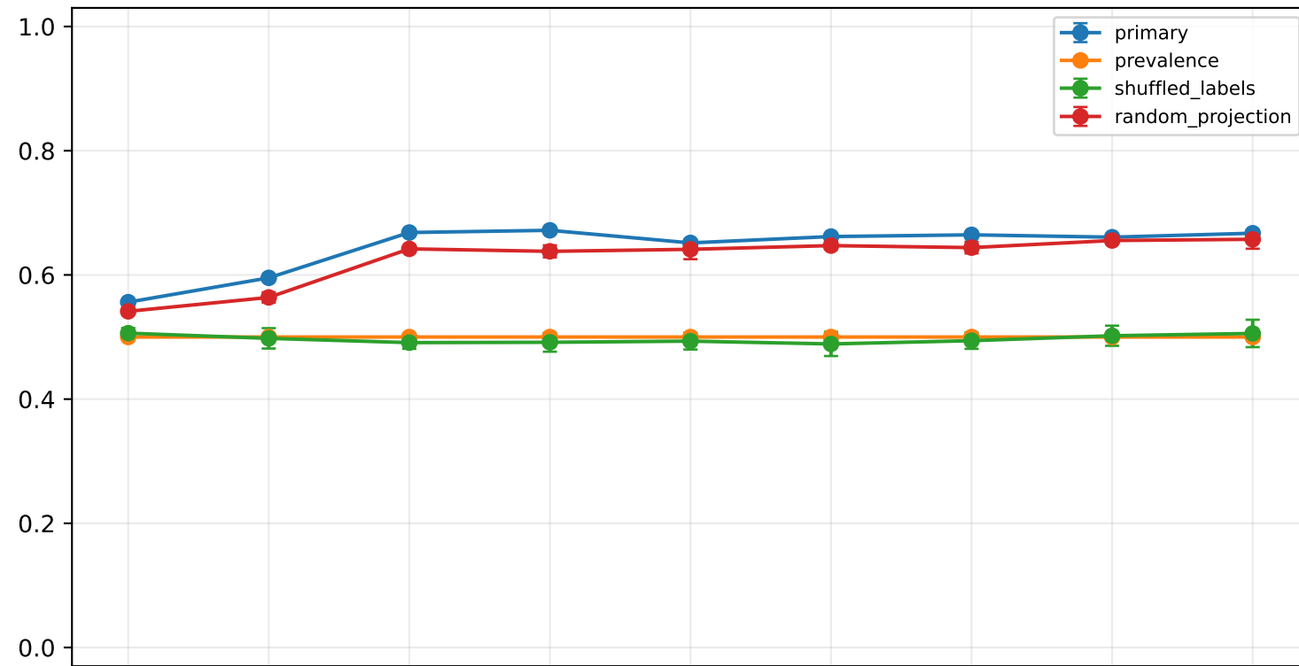
Macro AUROC: mean \pm seed SD
