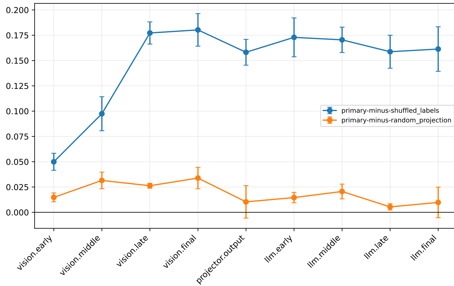
Paired AUROC differences: mean \pm seed SD
