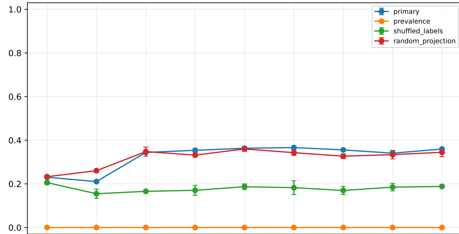
Macro F1: mean \pm seed SD
