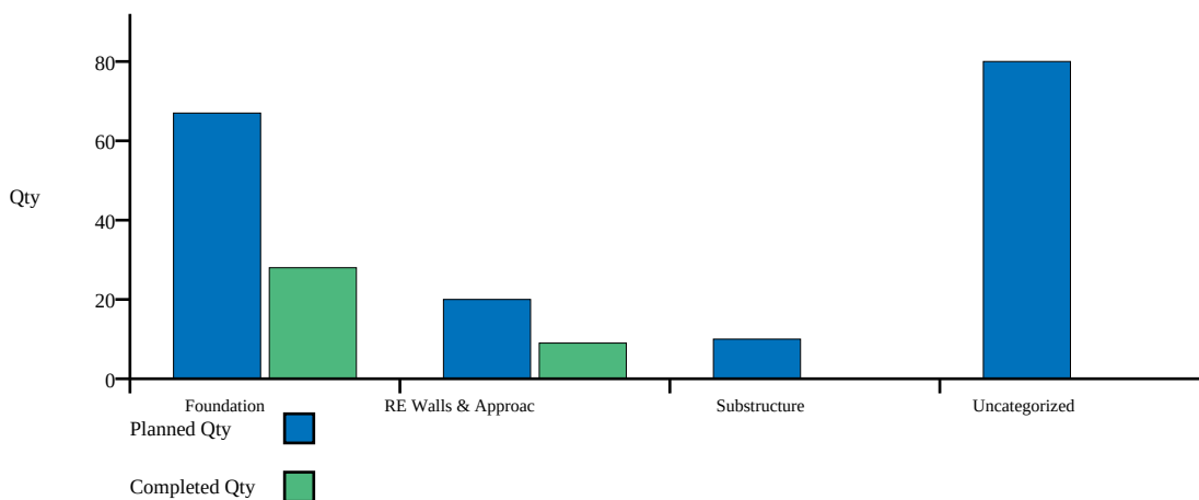
Scope Progress by Category (Quantity)
