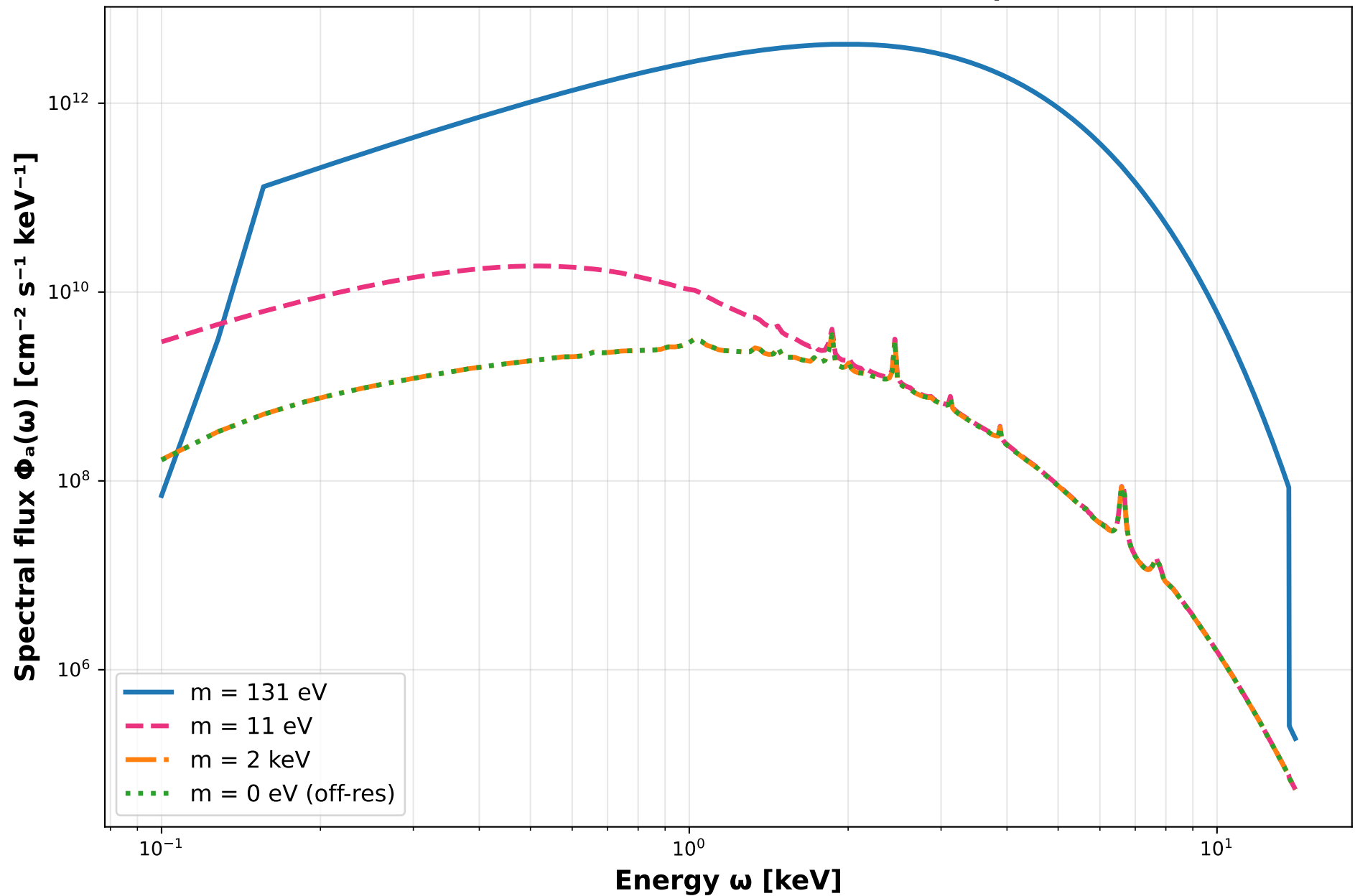
Transverse Plasmon Resonance: Axion Mass Dependence
